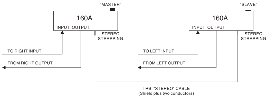
Figure 6: Multi-Channel Connections
